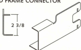
HD FRAME CONNECTOR
